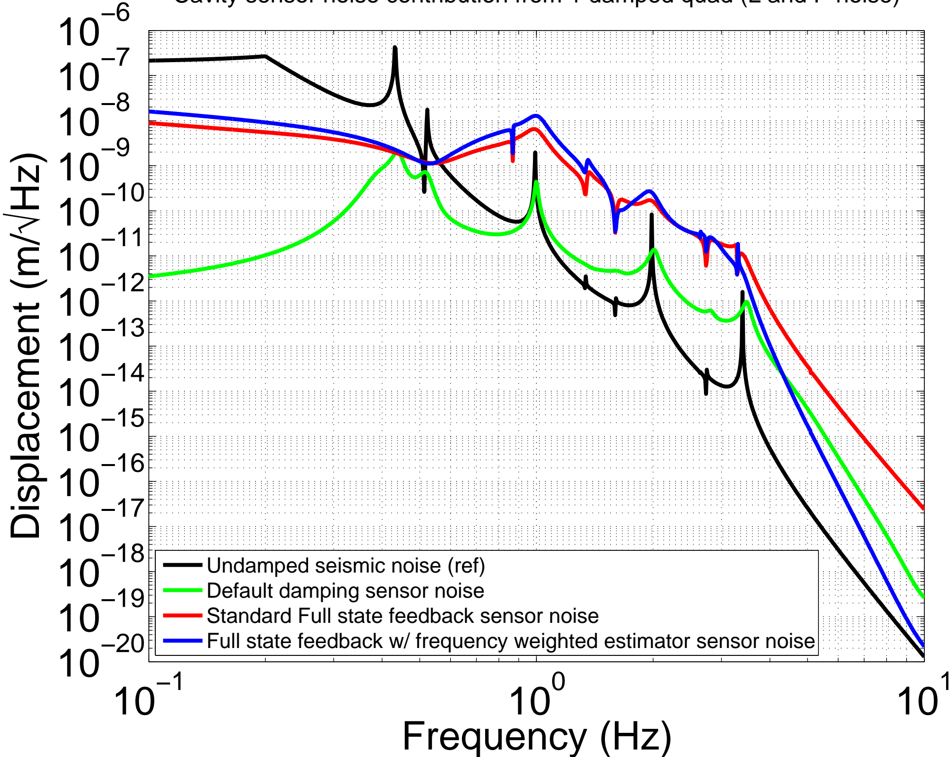
Cavity sensor noise contribution from 1 damped quad (L and P noise)
