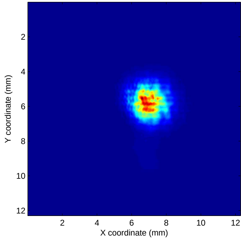
Pick-off beam incident on the HWS without the Hartmann plate
