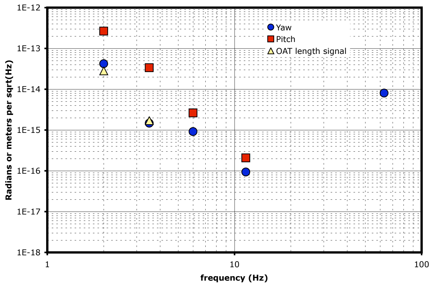
Predicted ITMY motion from ambient magnetic fields during science runs
