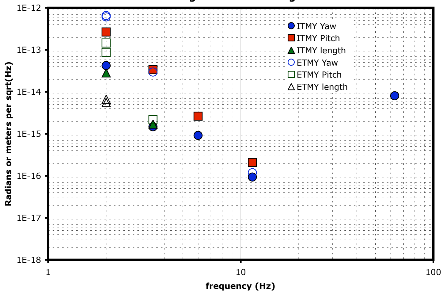
Predicted ITMY and ETMY motion from ambient magnetic fields during science runs
