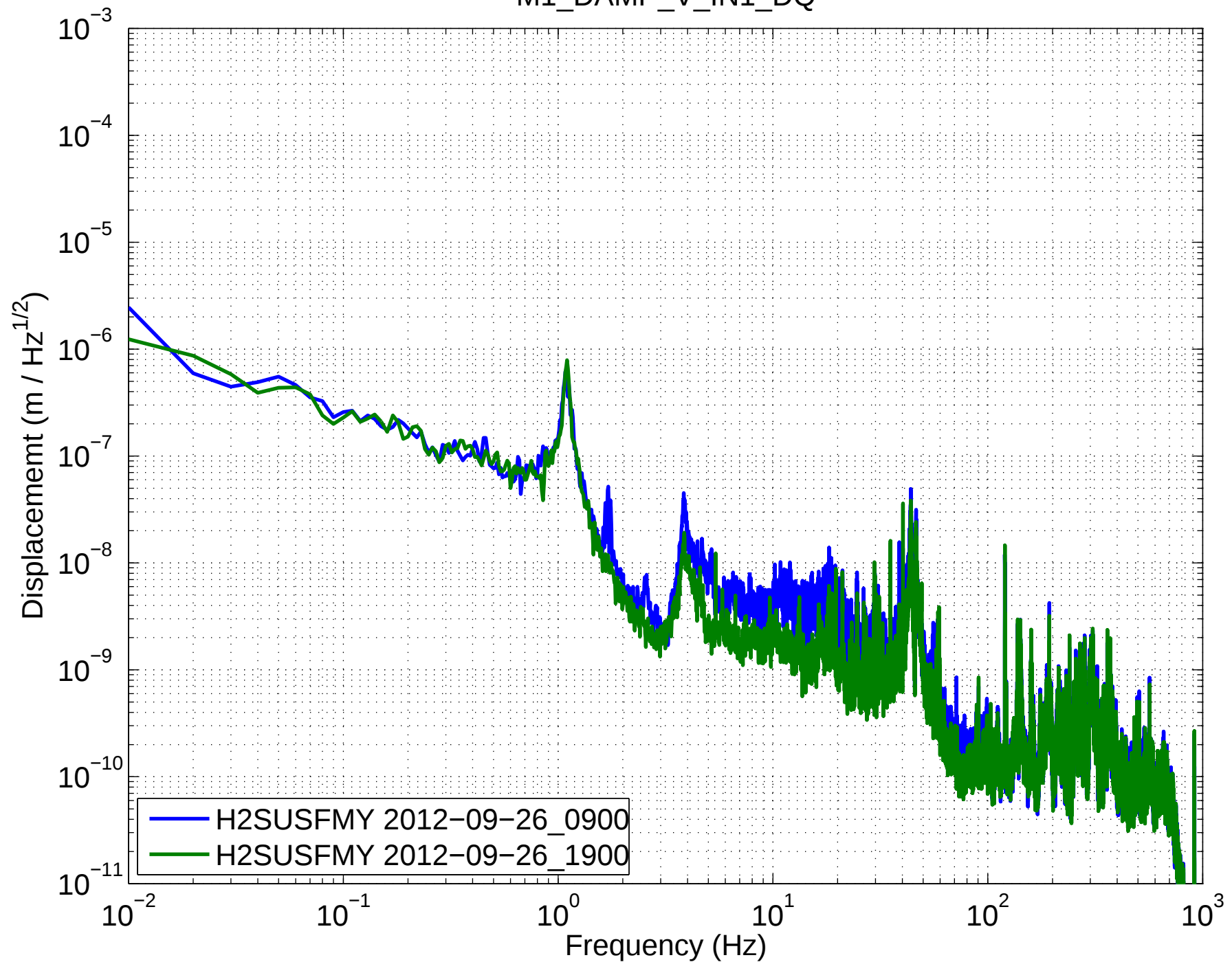
(BSFM) Amplitude Spectral Density – Damping ON M1_DAMP_V_IN1_DQ
