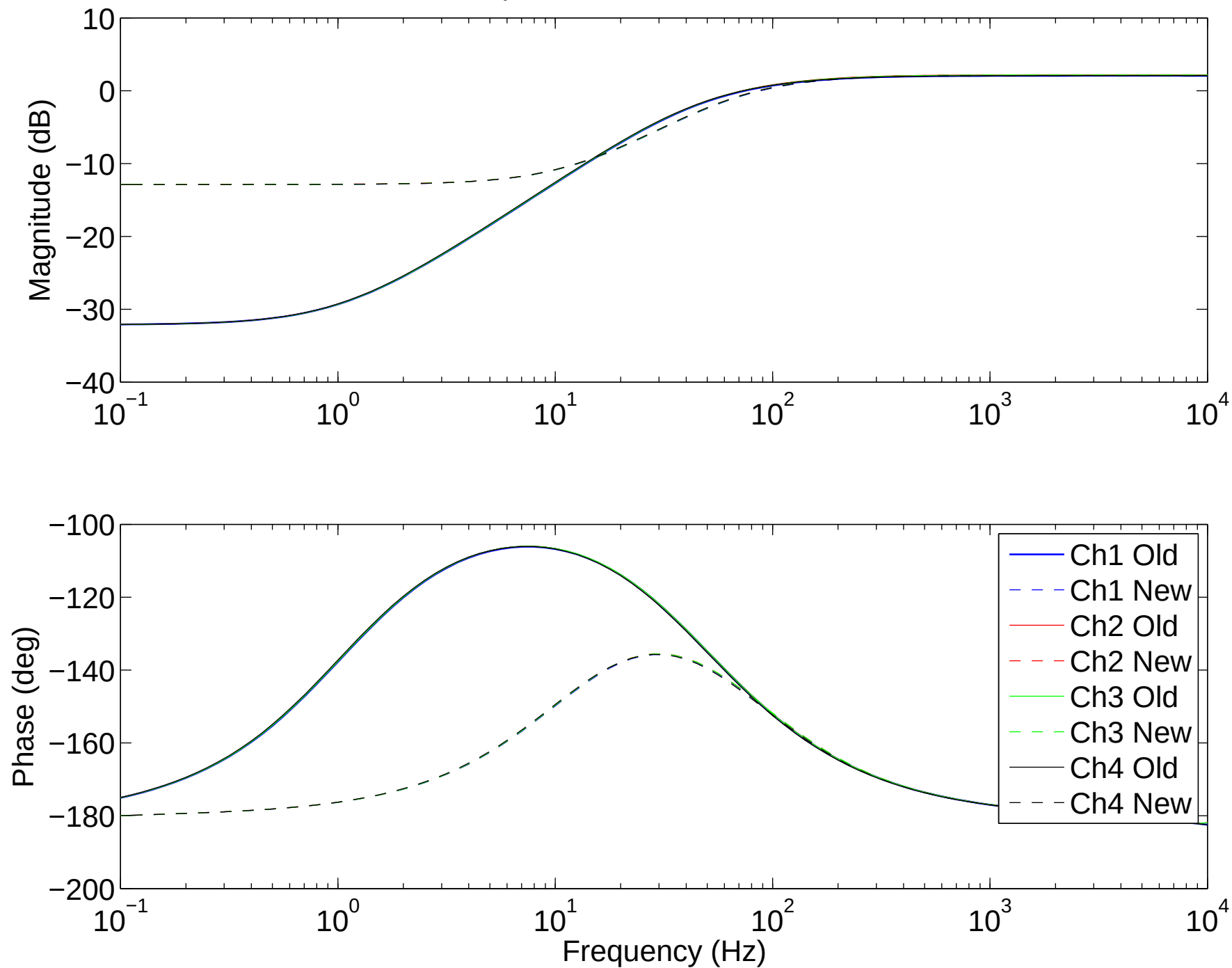
Acquire State Transfer Function
