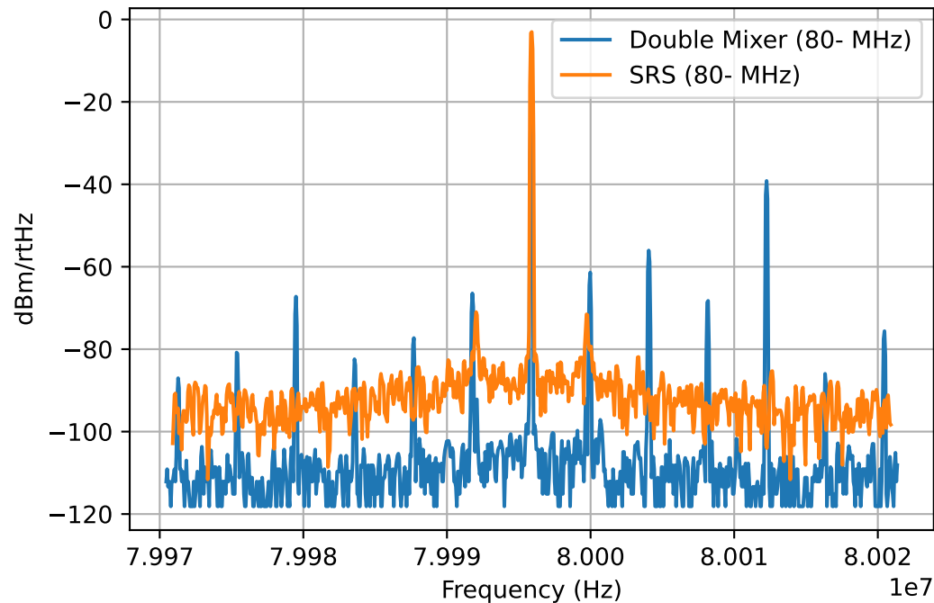
Double Mixer Spectrum 50kHz Span
