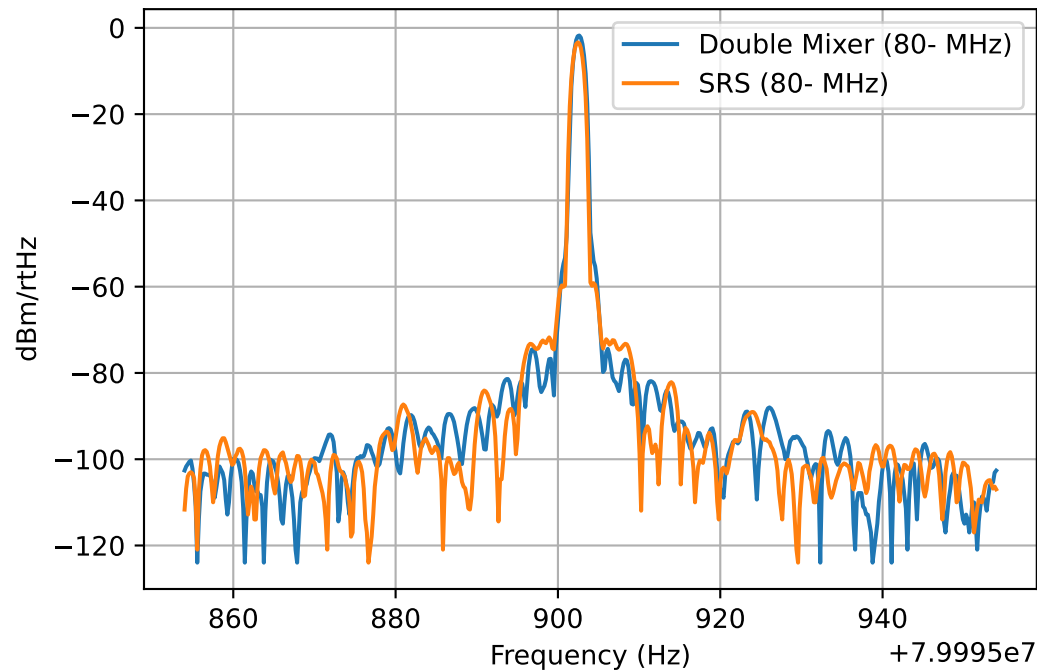
Double Mixer Spectrum 100Hz Span
