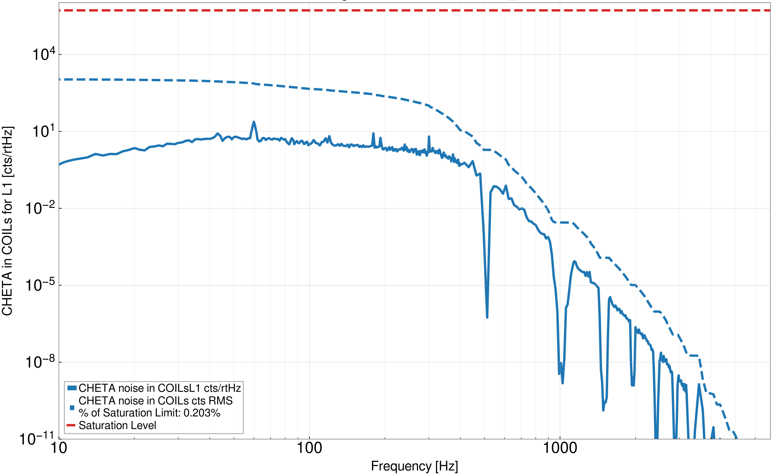
Calibrating \delta I_{CHETA} to counts before L1_DAC
