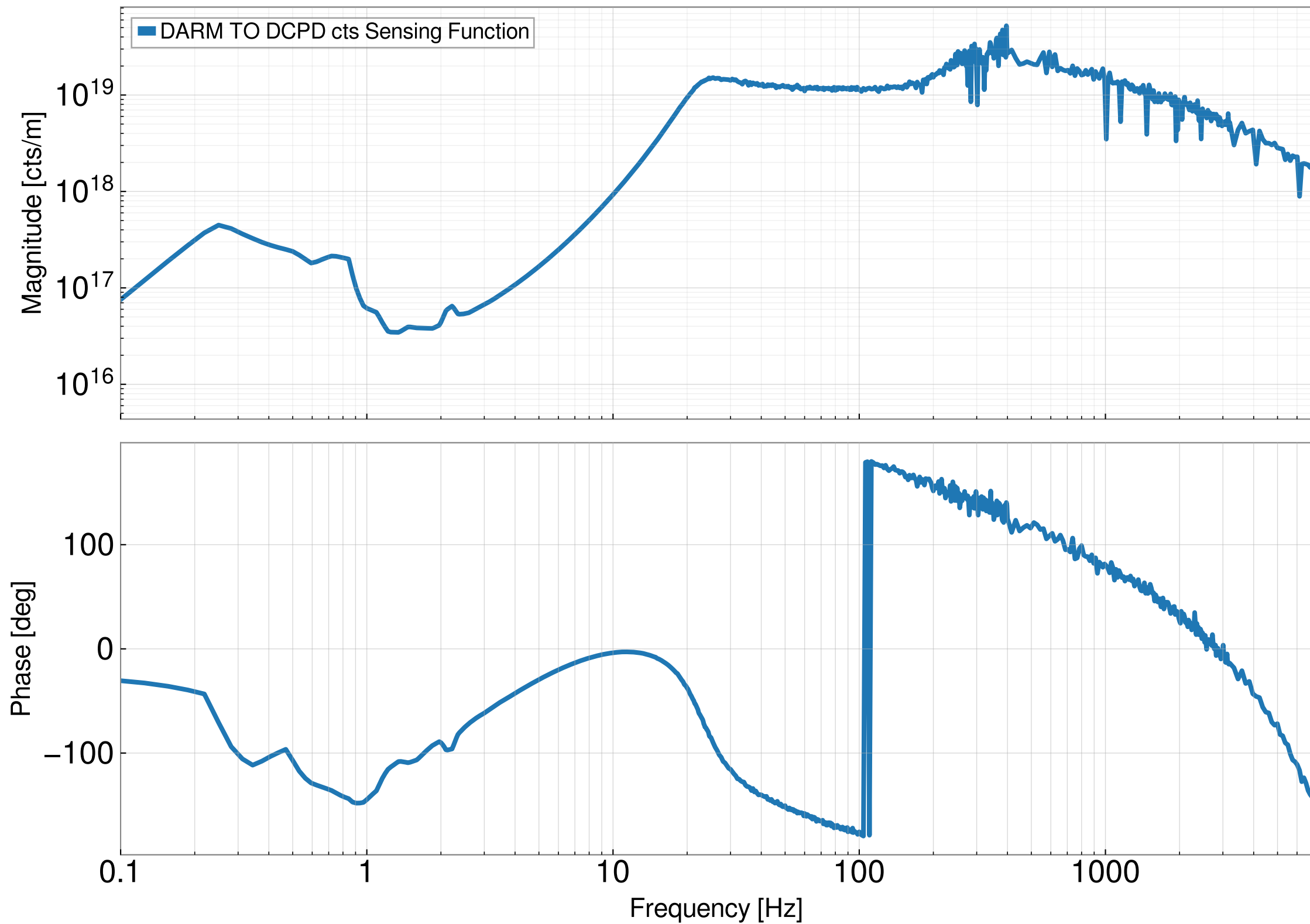
DARM to DCPD cts Trans. Func. Measurement 2025-01-23 T21:11:18
