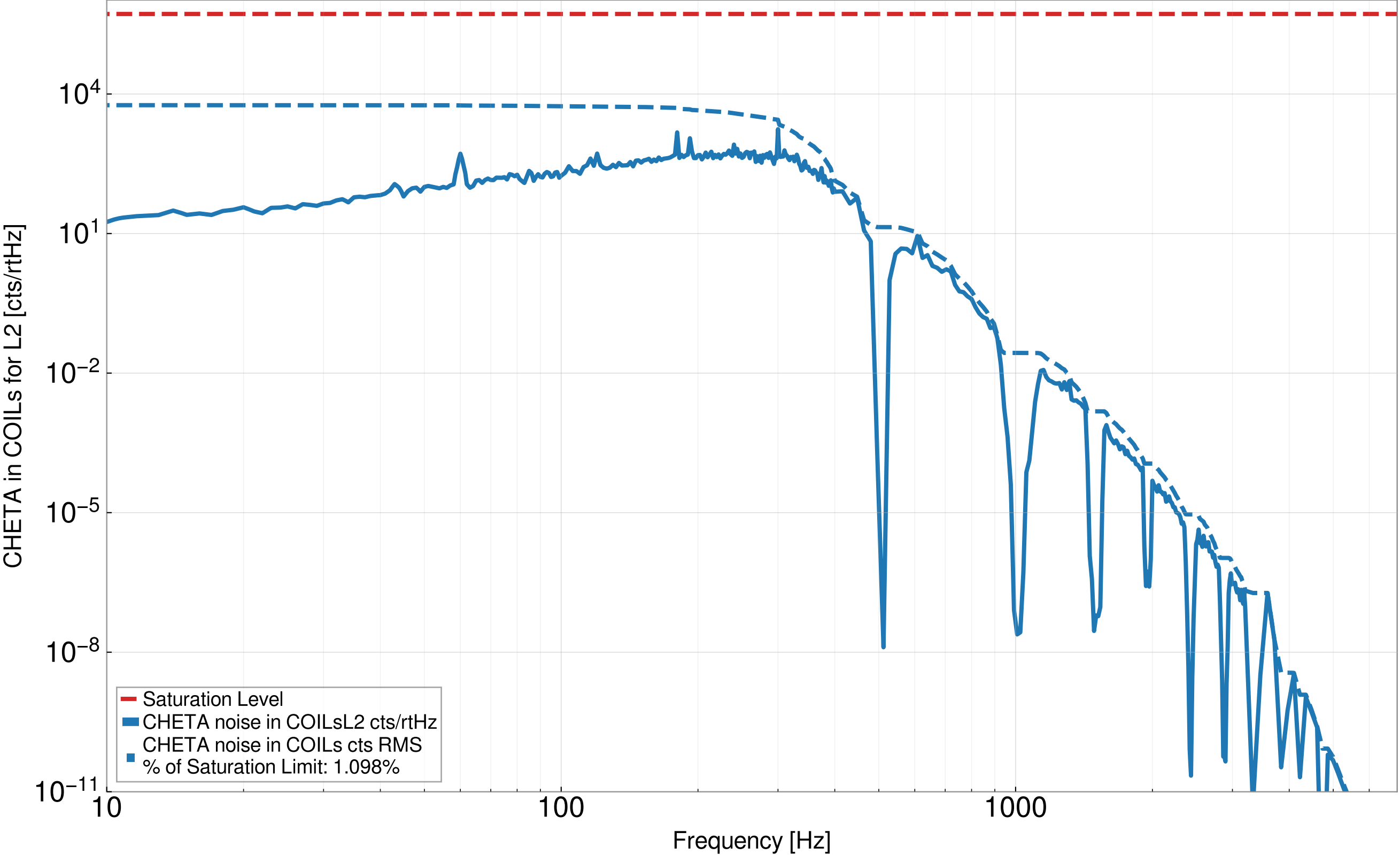
Calibrating \delta I_{CHETA} to counts before L2_DAC
