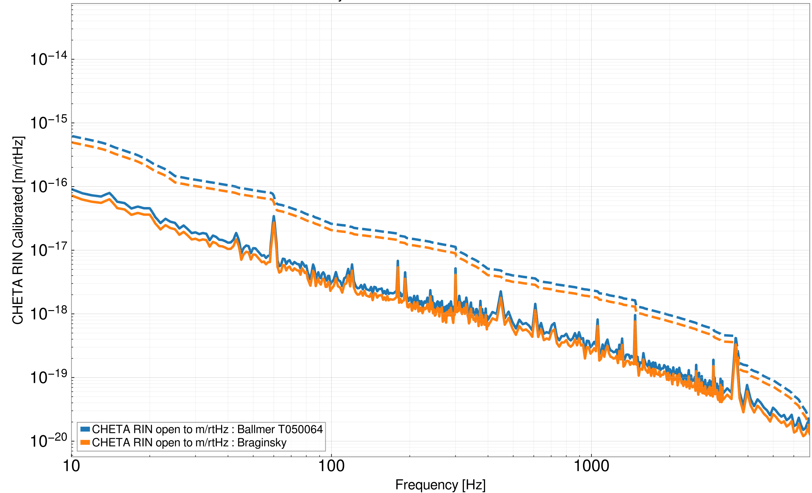
Relative Intensity Noise of CHETA CO2 Laser Calibrated to DARM
