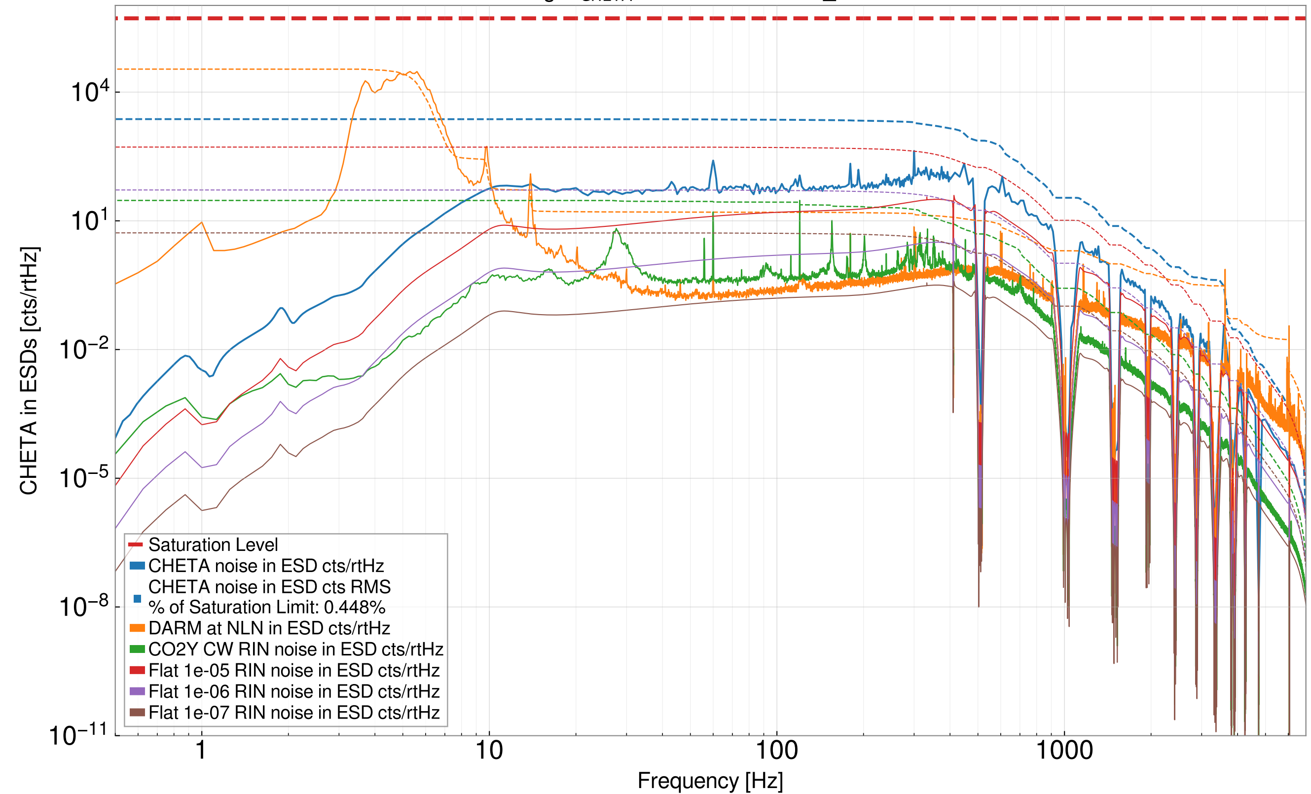
Calibrating \delta I_{CHETA} to counts before L3_DAC : P = 1W
