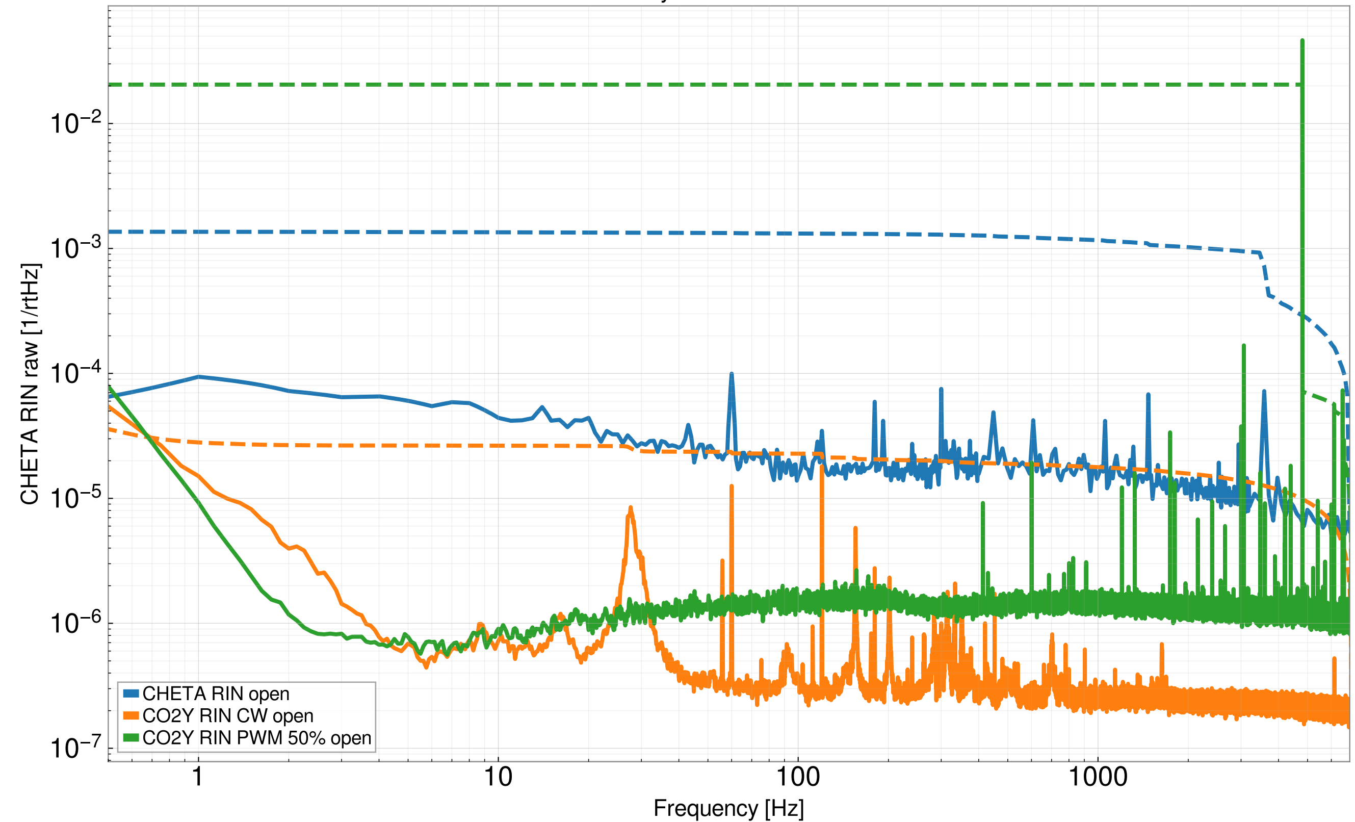
Relative Intensity Noise of CHETA CO2 Laser
