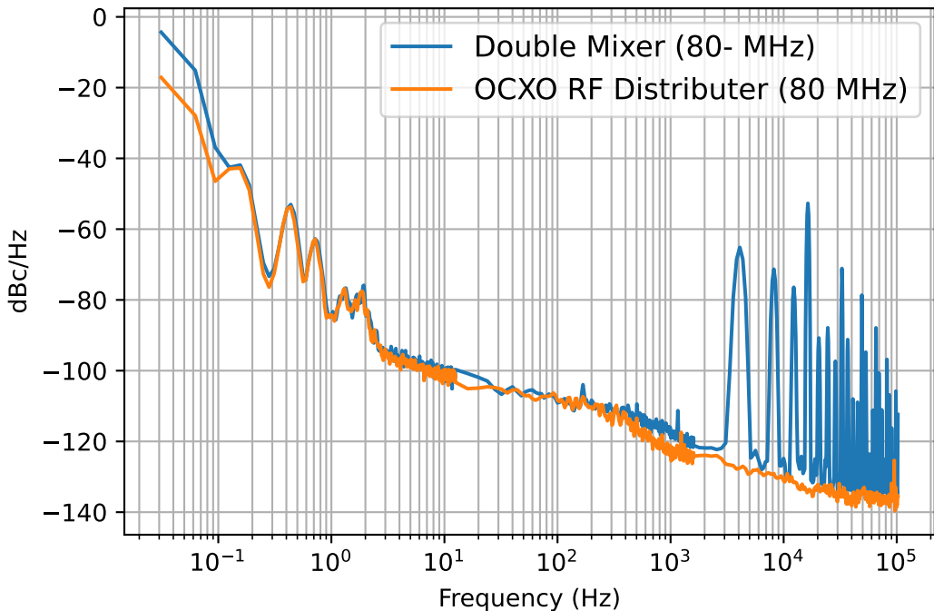
Double Mixer vs RF Distributer (Reference SRS SG382)
