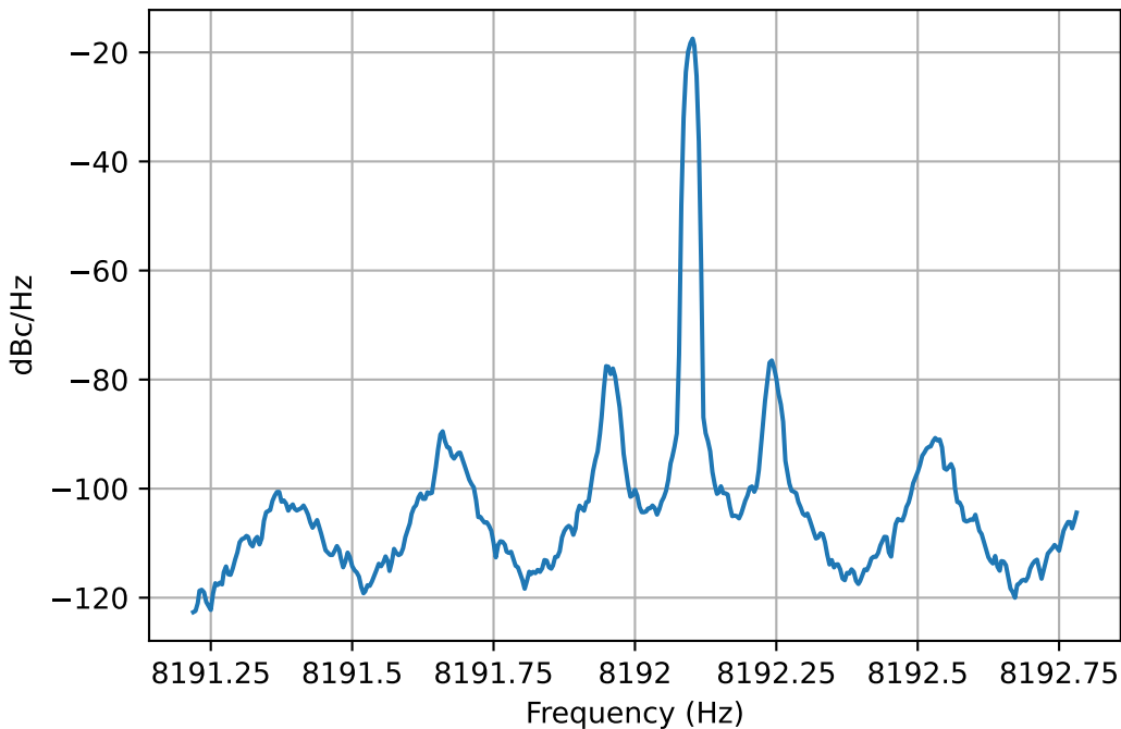
Zoom on Double Mixer 8kHz Sideband(3.9mHz div.)
