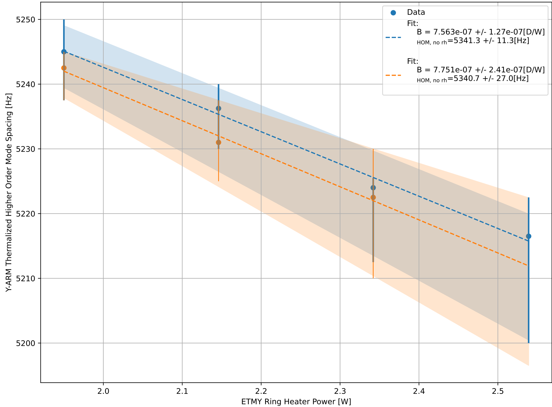
HOM Spacing vs. Ring Heater Power
