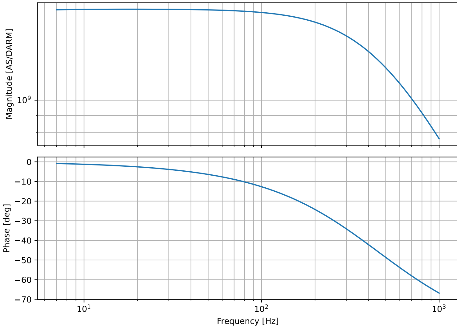
DARM input->DARM readout vs SRCL detuning
