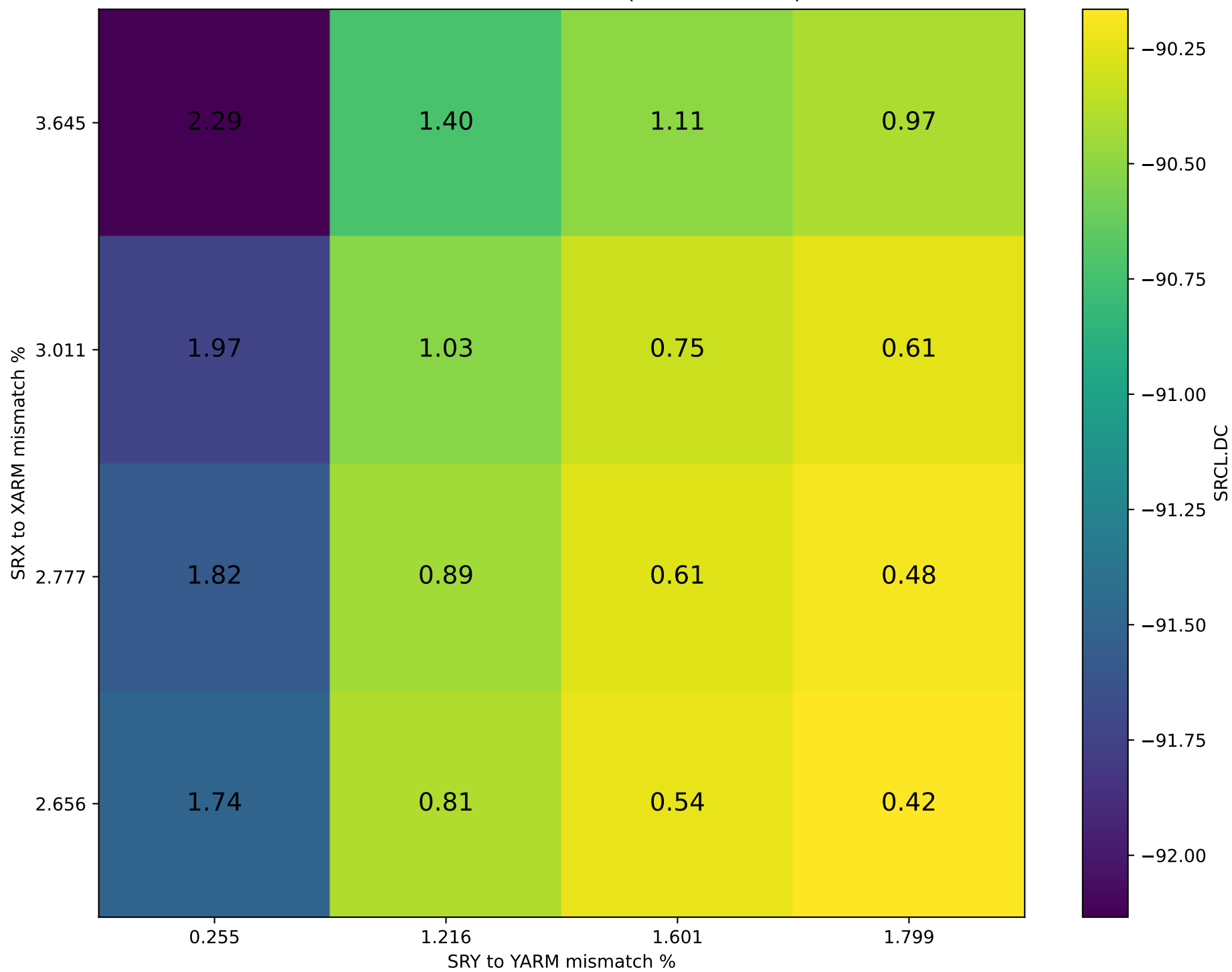
SRCL.DC vs Mode Mismatch (XARM vs YARM)
