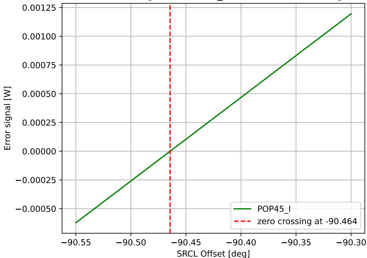
SRCL error signal at POP45_I with SRCL.DC detuning
