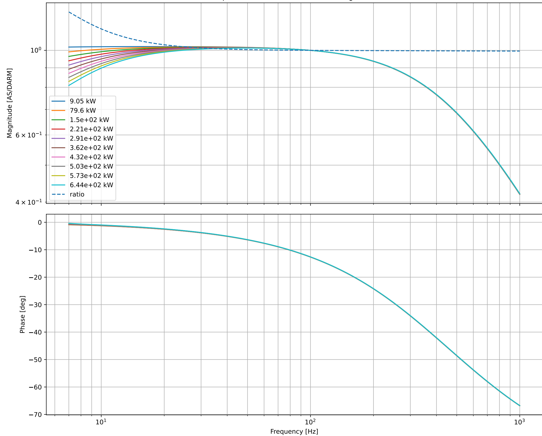
DARM input->DARM readout vs Circulating ARM Power
