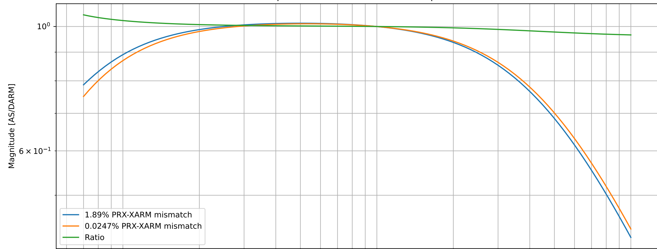
DARM input-&gt;DARM readout vs at 60.0 Input Power
