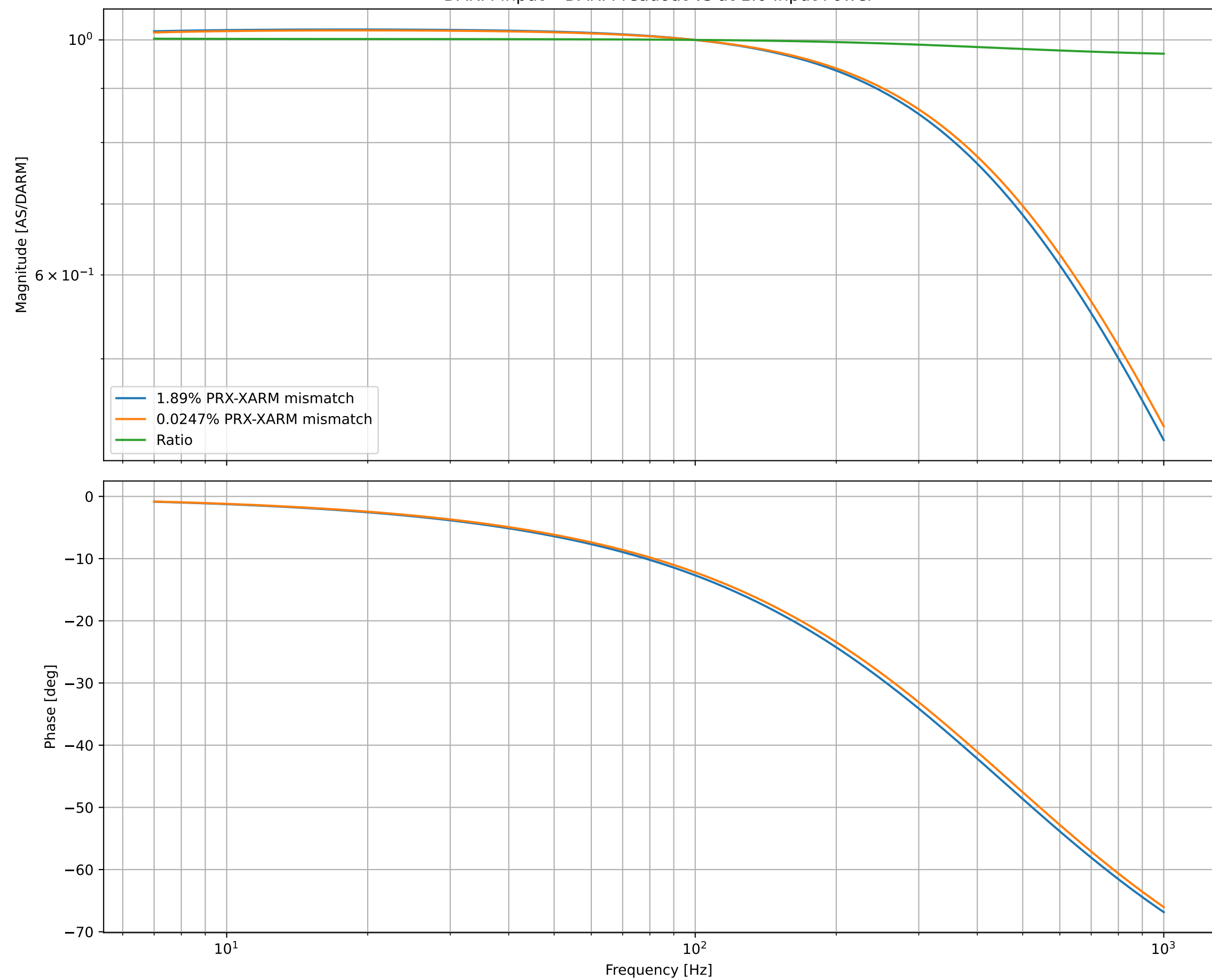
DARM input-&gt;DARM readout vs at 1.0 Input Power
