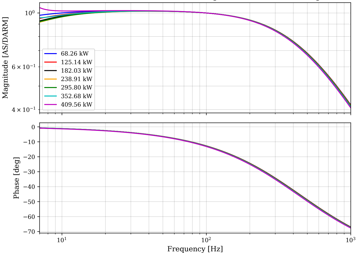
Thermal Distortion Effects on DARM Sensing Function with Circulating Power
