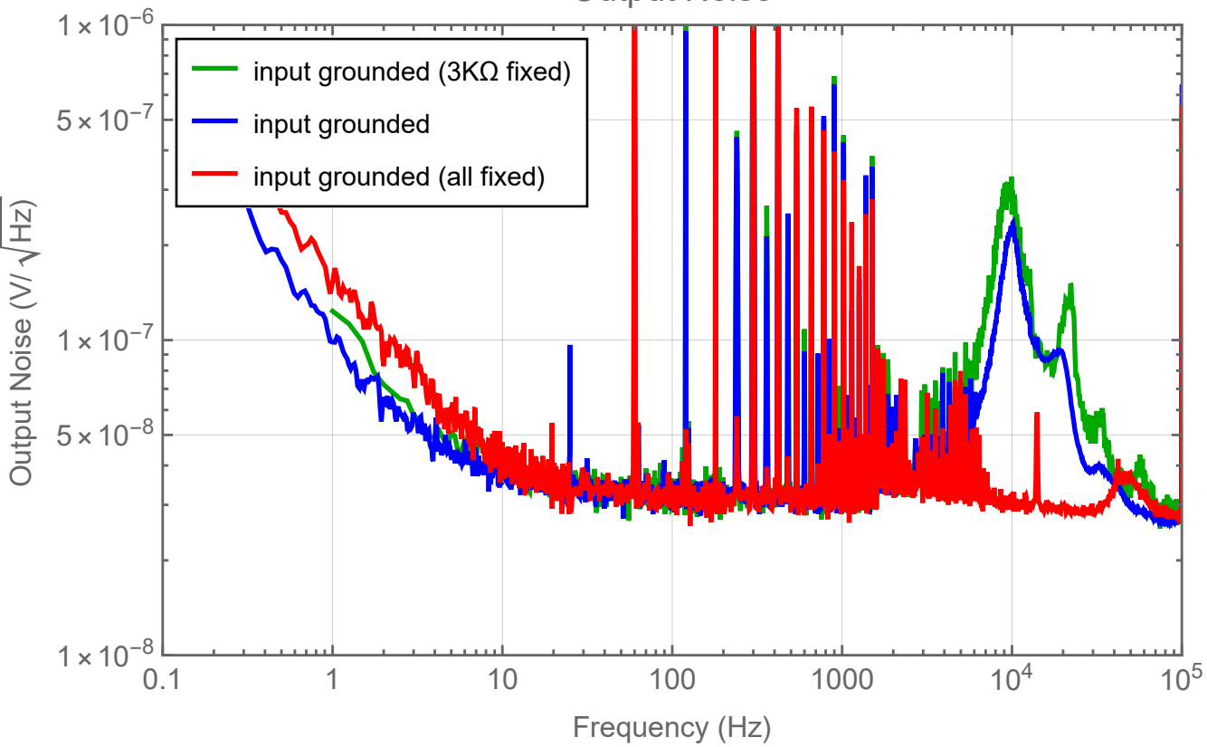
Output Noise
