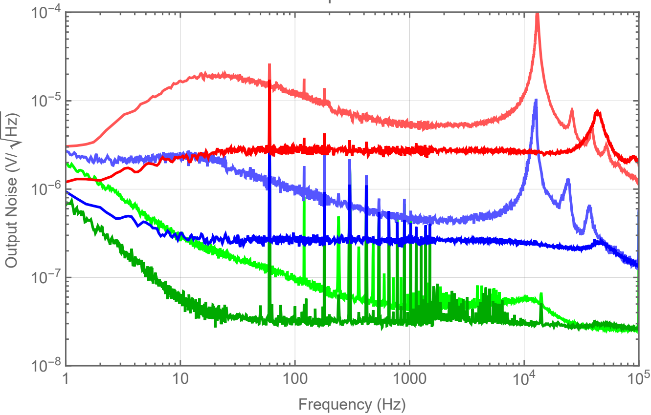
Output Noise
