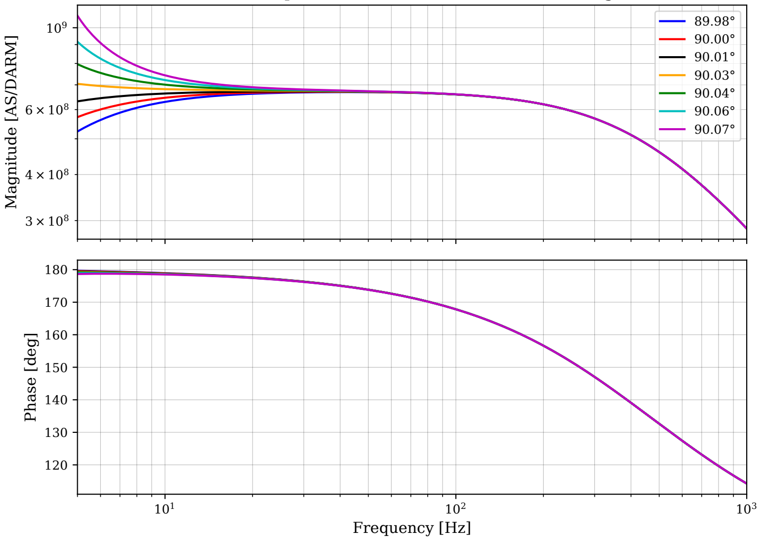
DARM input \rightarrow DARM readout vs SRCL detuning
