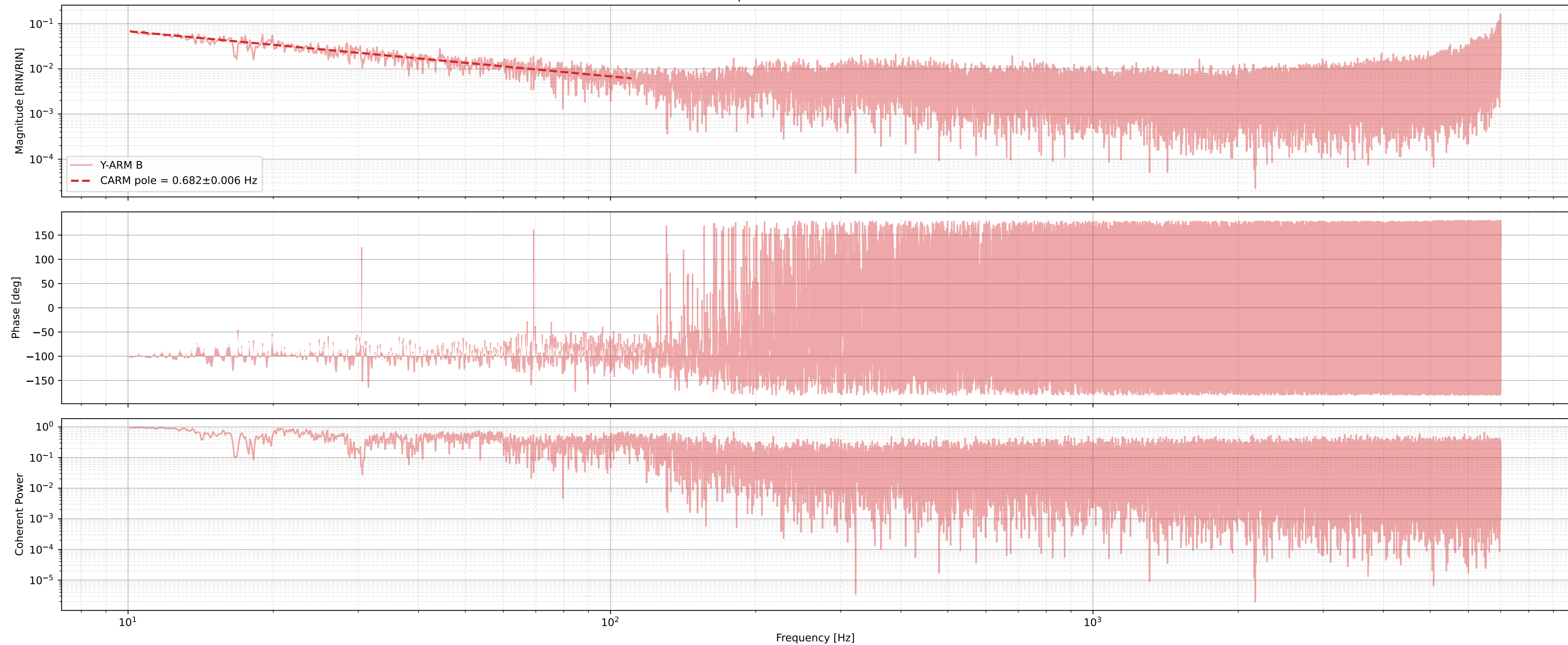
Input RIN to Y-ARM B RIN fits
