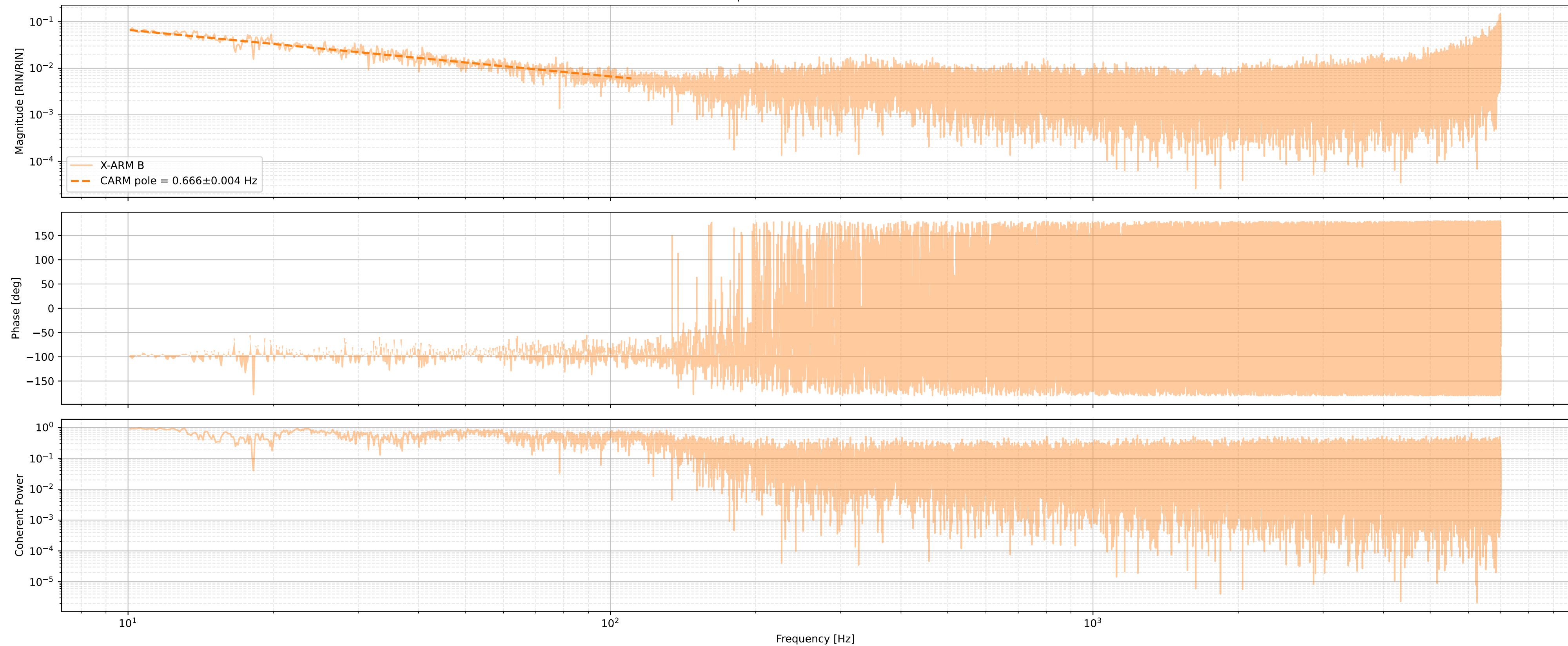
Input RIN to X-ARM B RIN fits
