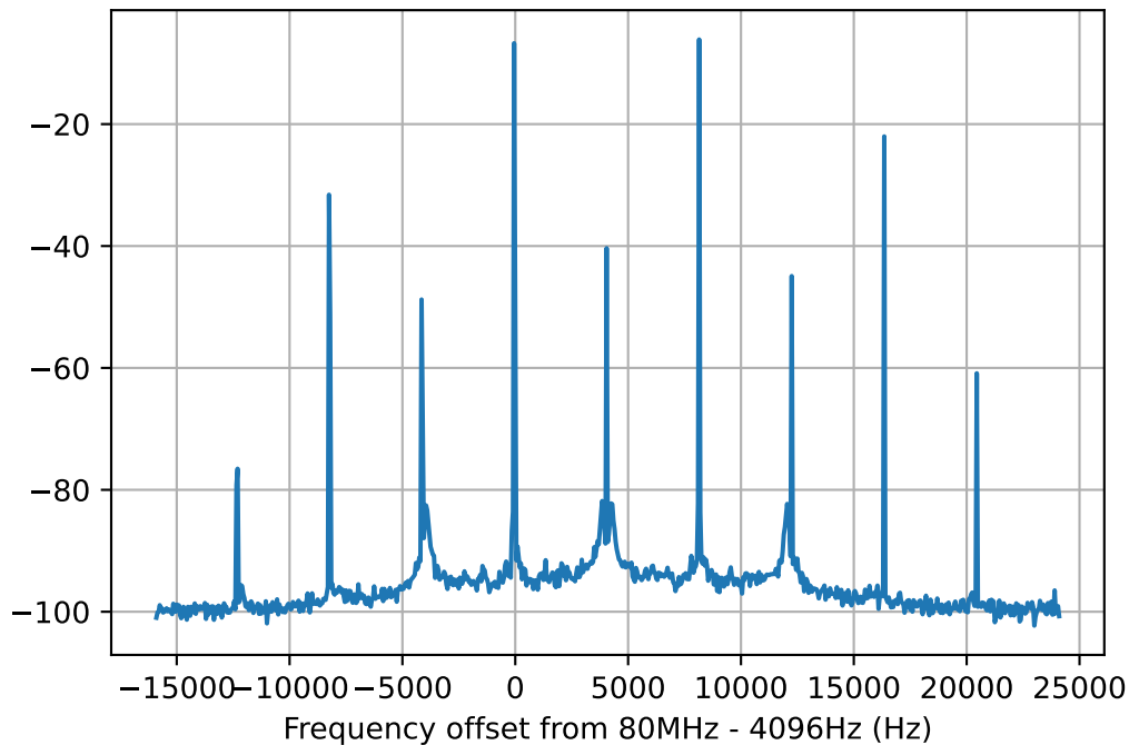
ZLW-1BR Spectrum 20kHz Span
