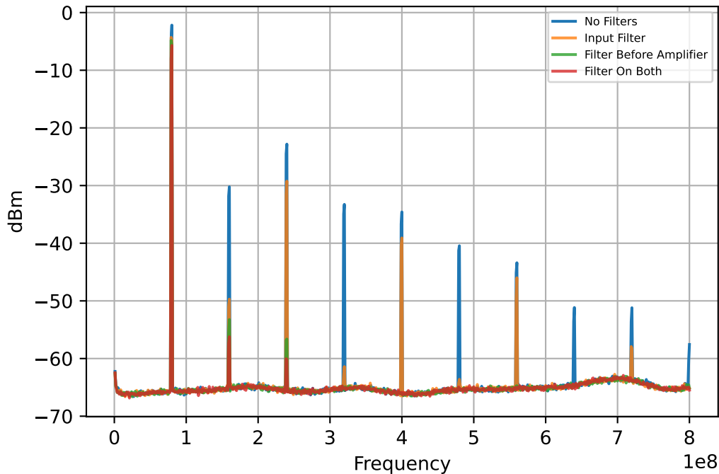
Double Mixer Spectrum 400MHz Span Filter Comparison
