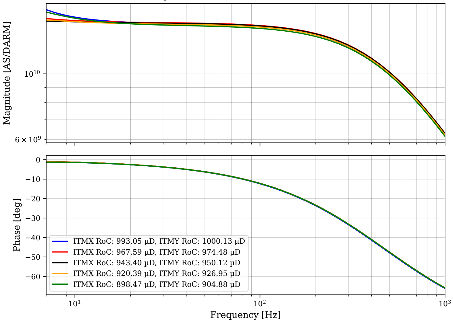
DARM input->DARM readout at Common ITM RoC
