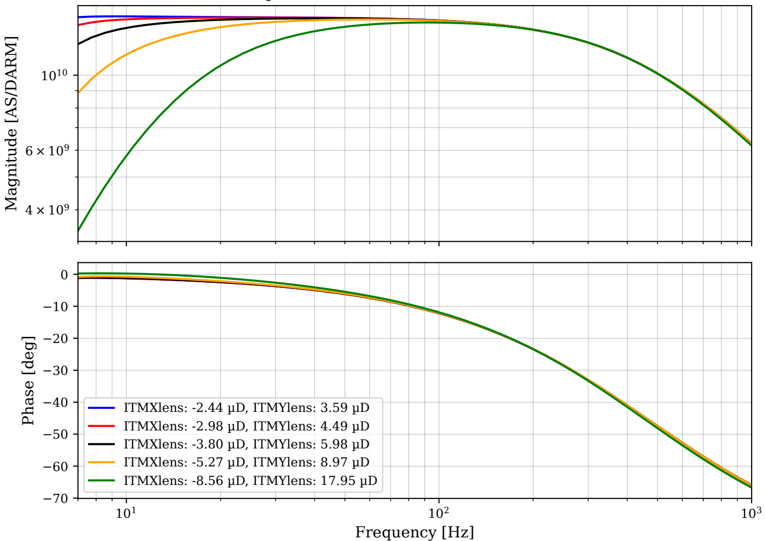
DARM input->DARM readout at Differential ITM lens
