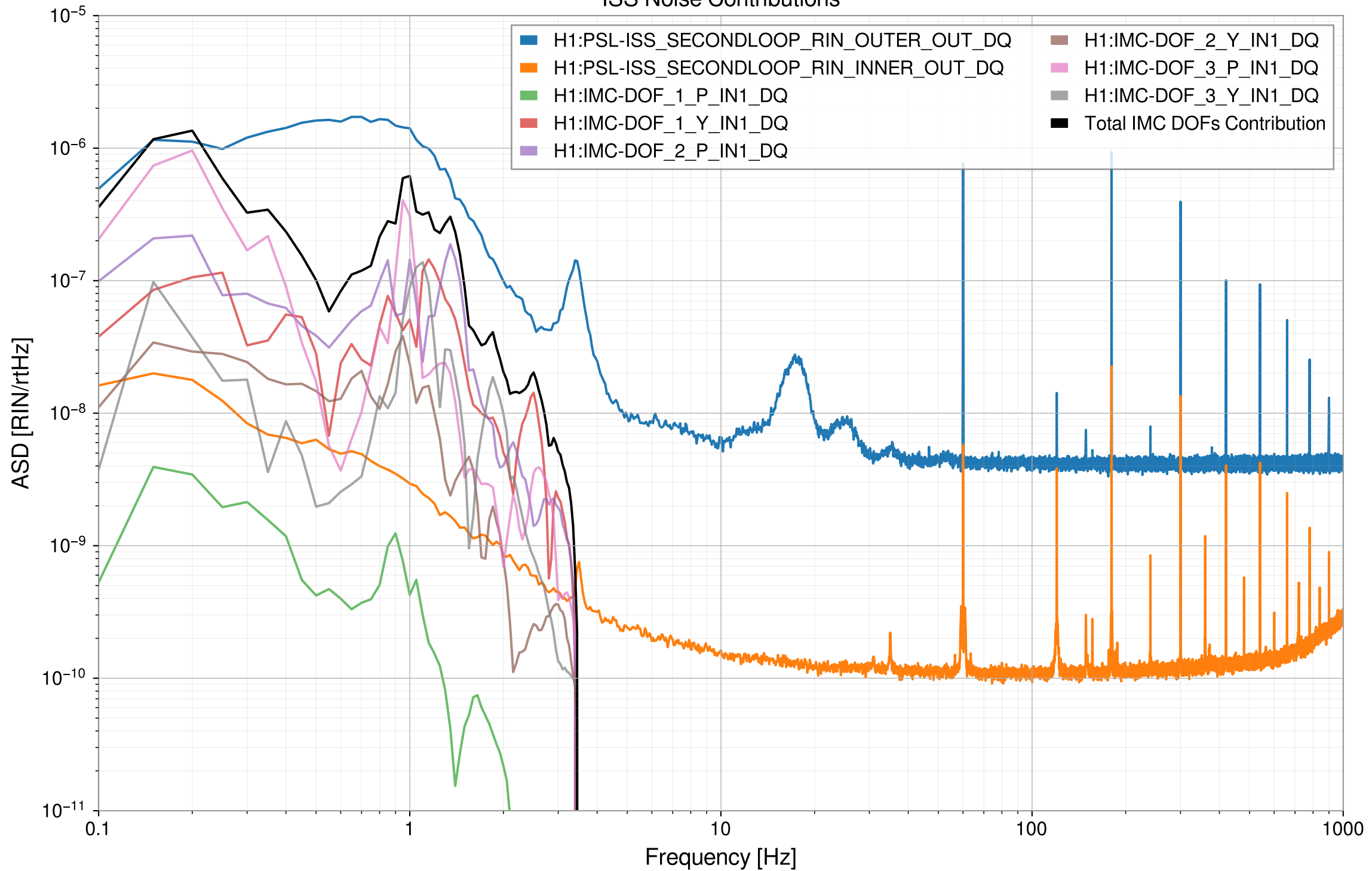
ISS Noise Contributions
