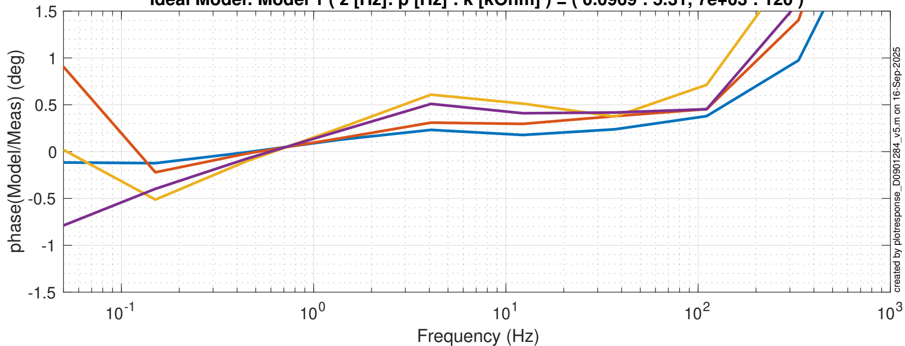
Ideal Model: Model 1 ( z [Hz]: p [Hz] : k [kOhm] ) = ( 0.0969 : 5.31, 7e+03 : 120 )
