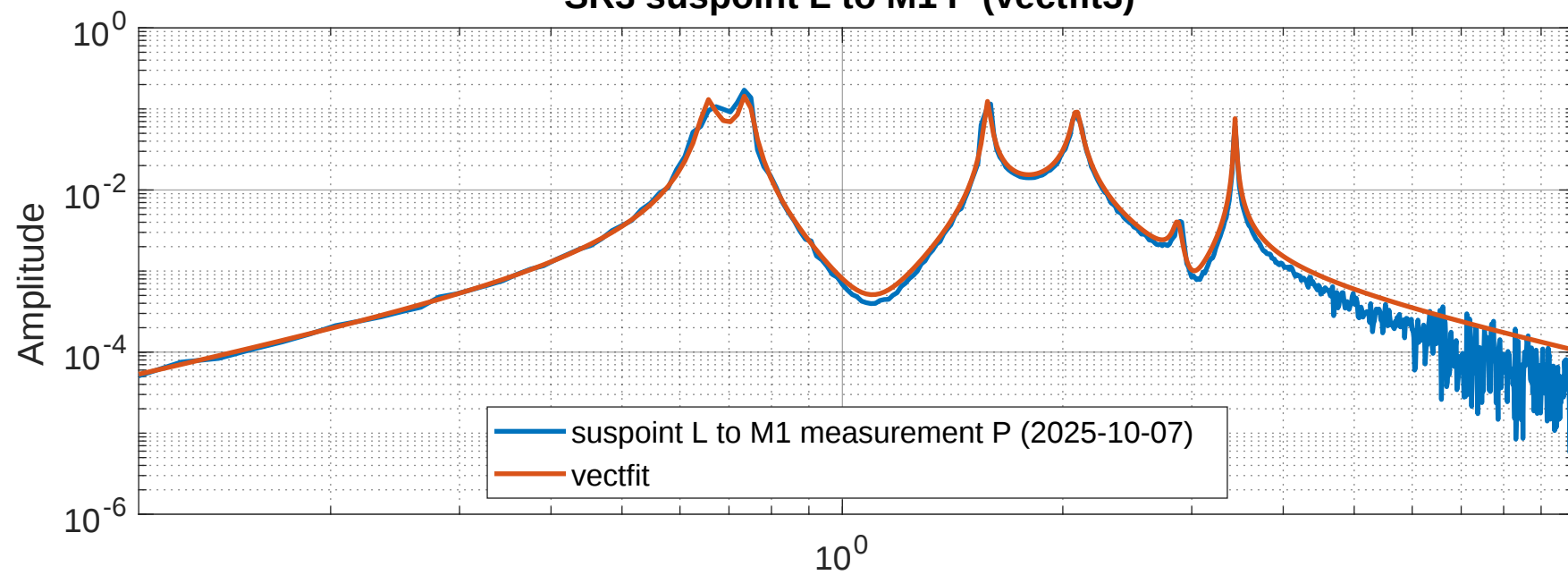
SR3 suspoint L to M1 P (vectfit3)
