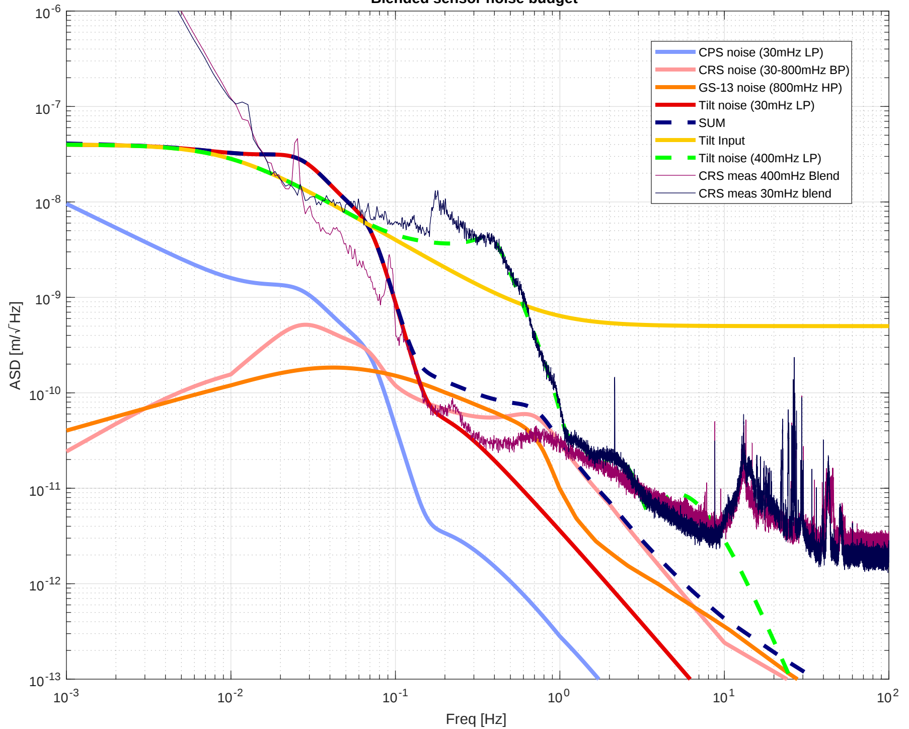
Blended sensor noise budget
